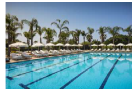
Activity Pool
